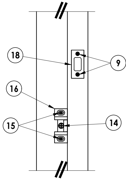
ROLLER LATCH & DEADBOLT STRIKE DETAIL
